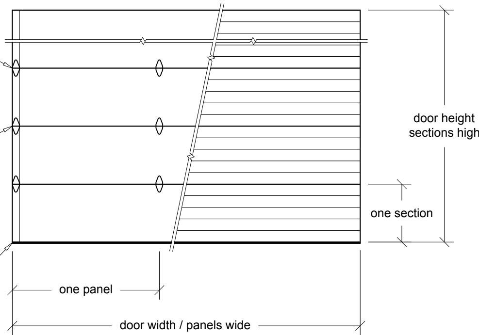
Interior Elevation
