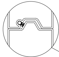
Joint Detail Tongue and groove design With weather seal
